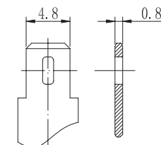
Terminal T1
